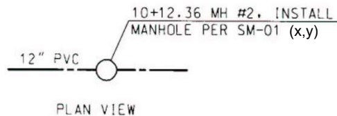
Figure 6.2.1 Manhole Plan Callouts
