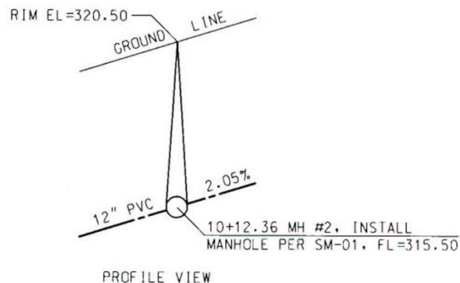
Figure 6.2.2 Manhole Profile Callouts
